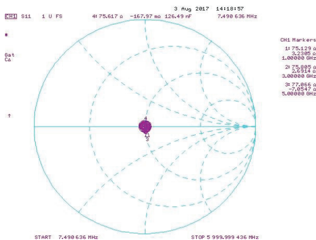
Smith Chart
